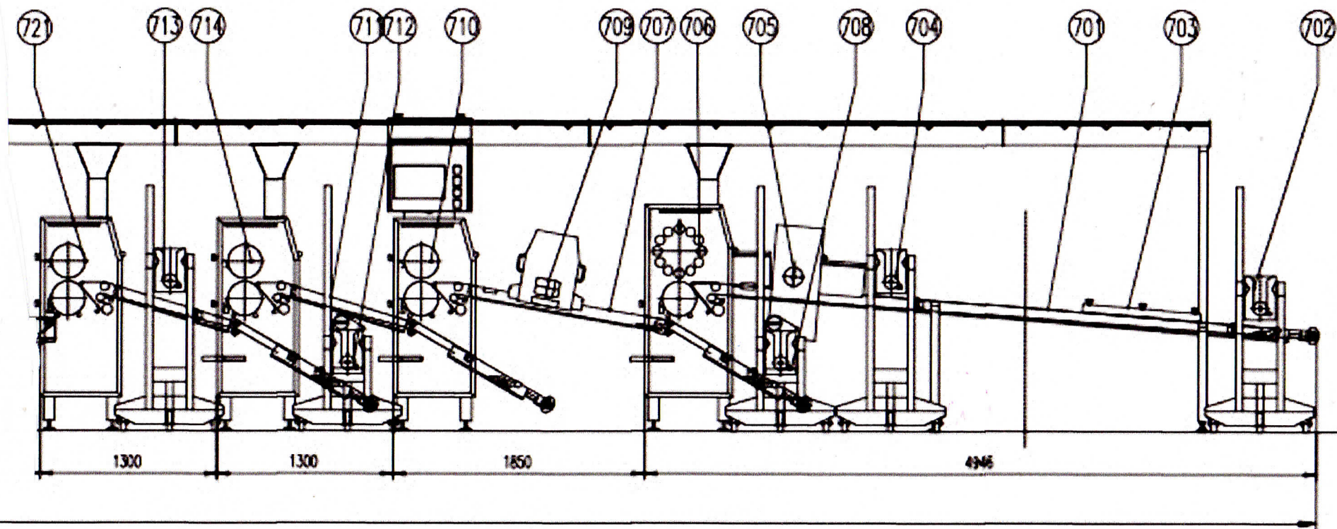
SHEETING LINE Working Width 800 mm.
