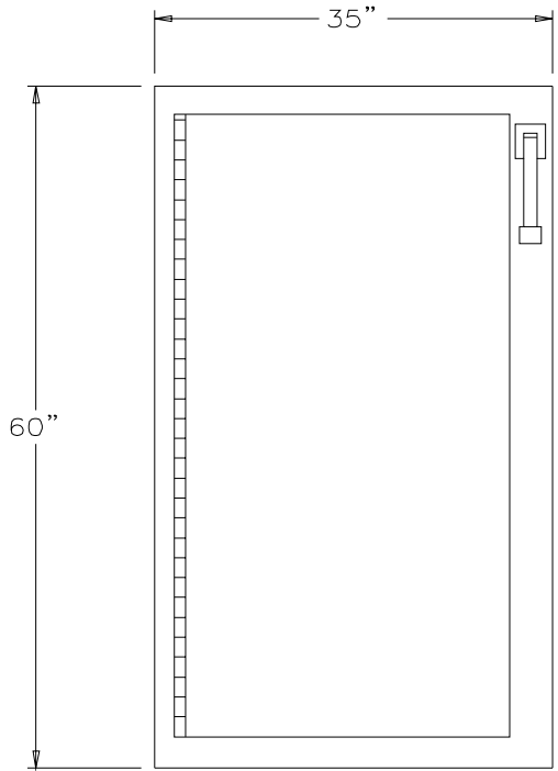
REMOTE MOUNTED NEMA 12 ELECTRICAL ENCLOSURES 12" DEEP
