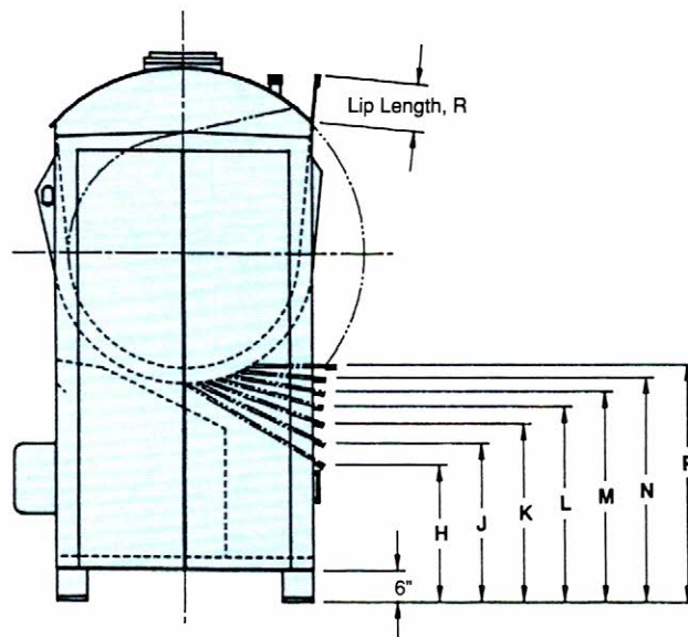
Tilt Height with Extended Lip
