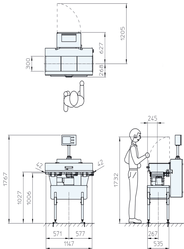
The Checkweigher Stand alone with controlpanel
