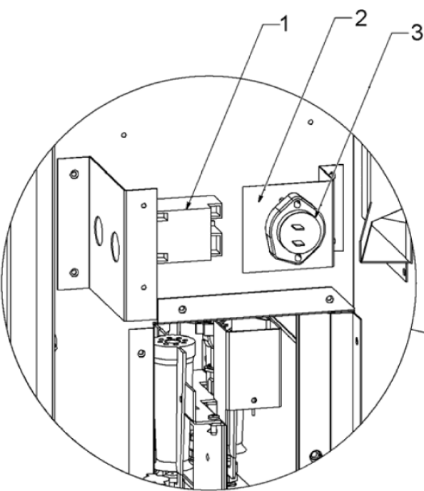
DETAIL B
