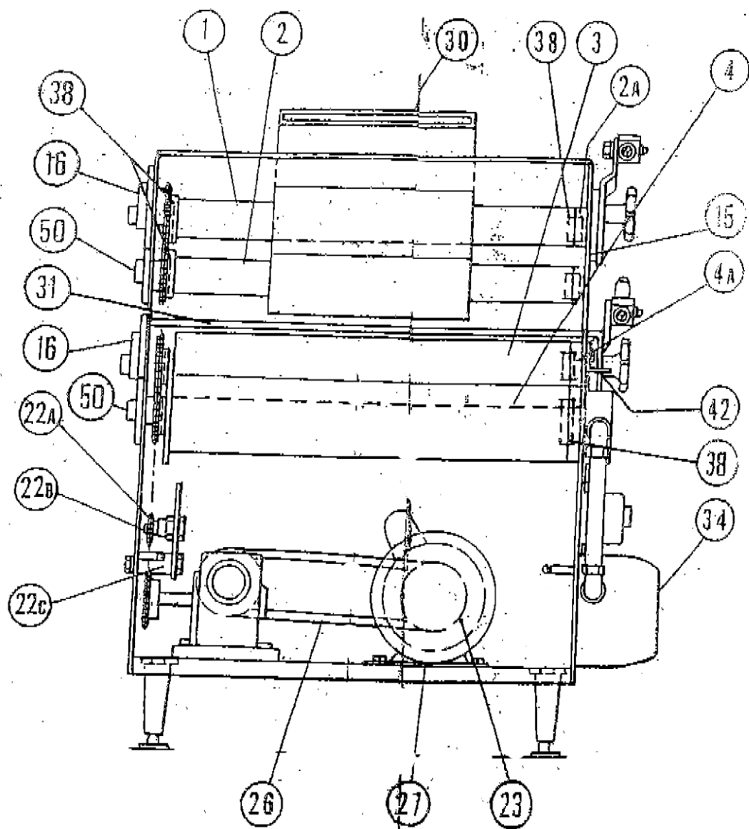
FRONT OR OPERATING SIDE (SLIDES & DRIVE GUARD REMOVED FOR CLARITY)
