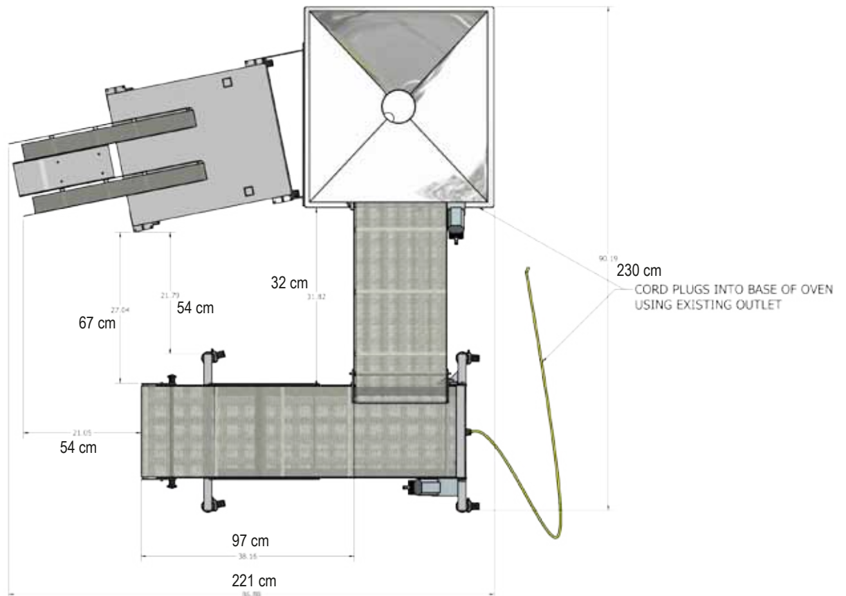
MODEL 20RX WITH 42" (107 CM) EXIT CONVEYOR AND RETURN CONVEYOR
