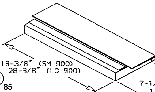
Deflector, Side
