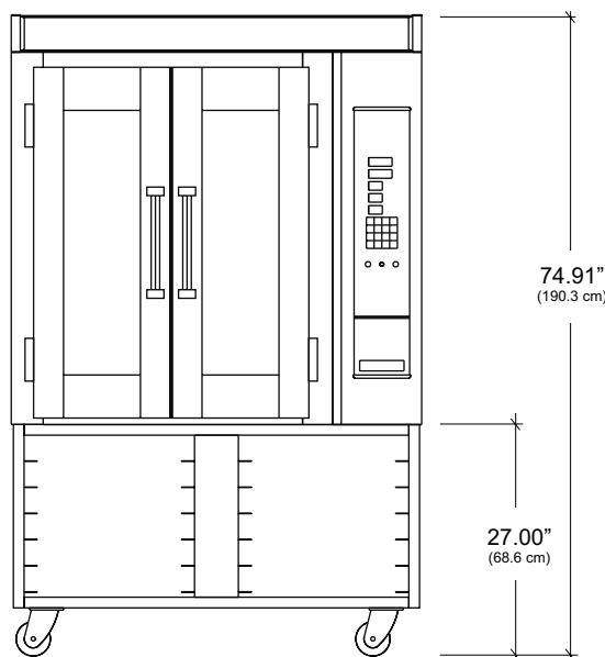
Height reflects OV300 with Standard Trim and 12-Pan Stand
