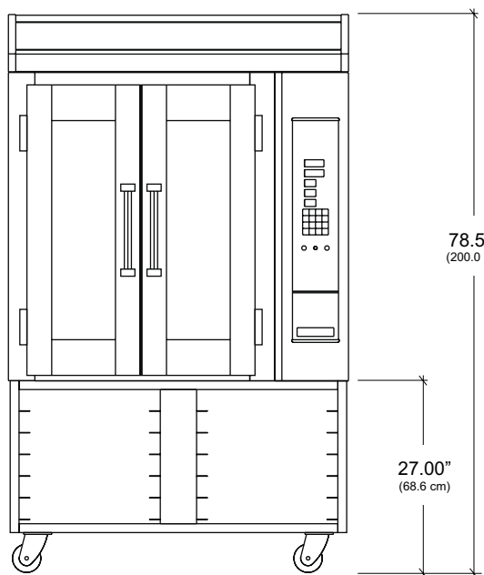
Height reflects OV300 with Optional Trim and 12-Pan Stand
