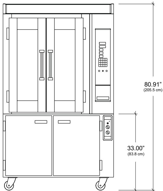
Height reflects OV300 with Standard Trim and 16-Pan Proofer or 16-Pan Stand
