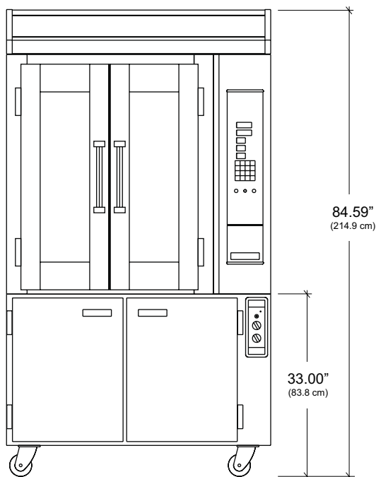
Height reflects OV300 with Optional Trim and 16-Pan Proofer or 16-Pan Stand
